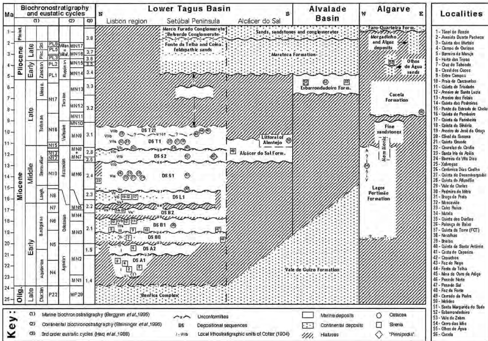
Fig. 5 - Stratigraphic distribution of marine mammal localities in the Neogene of Portugal. Continental biostratigraphy (2) and 3rd order eustatic cycles (3) correlated to marine biostratigraphy (1). Stratigraphic frameworks adapted from Antunes et al. (2000a) and Manuppella (1994) for the Lower Tagus Basin (Lisbon region and Setúbal Peninsula); Oliveira et al. (1992) for the Lower Tagus Basin (Alcácer do Sal) and Alvalade Basin; and Antunes et al. (2000b) for the Algarve.
