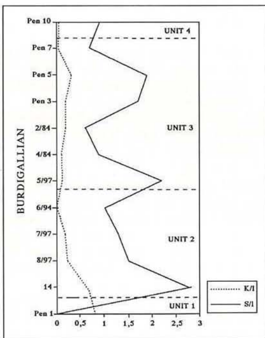
Fig. 9 - Penedo Sul: variations on the relative contents of the main clay minerals. K/I - Kaolinite/Illite; S/I - Smectite/Illite.
