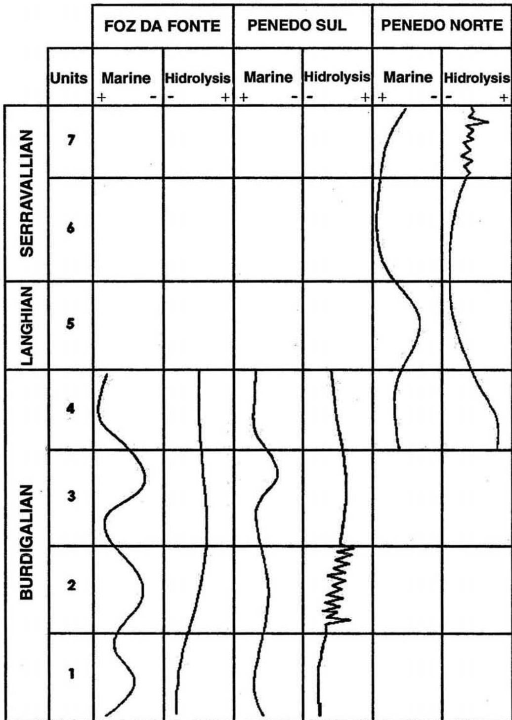
Fig. 21 - Paleoenvironmental evolution.
