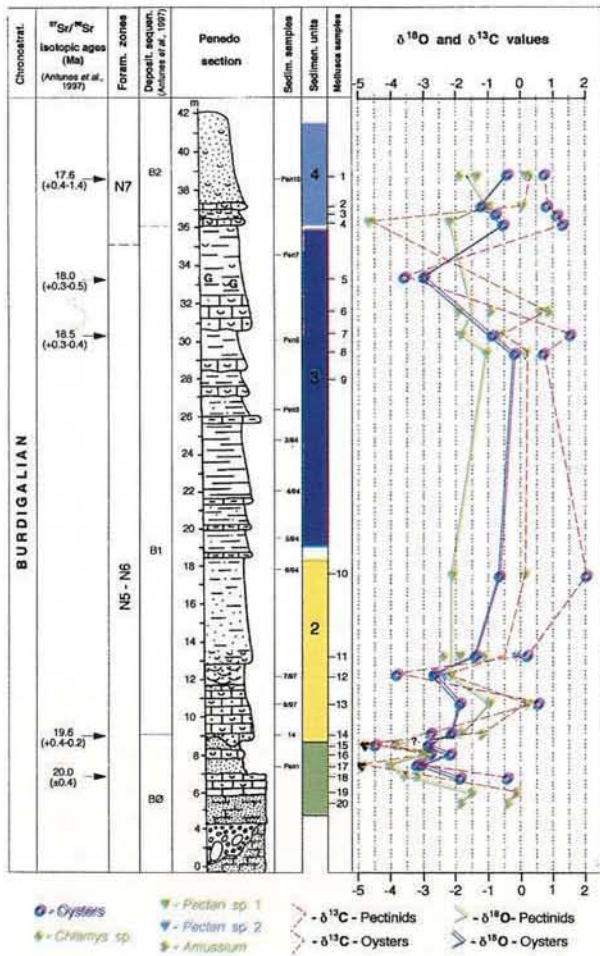
Fig. 8 - Penedo Sul Section, C and O isotopic composition (Antunes et al., 1997).
