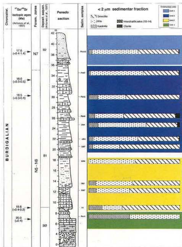
Fig. 7 - Penedo Sul Section. Composition of the <2µm sedimentary fraction.
