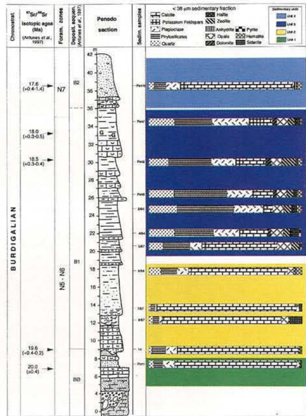
Fig. 6 - Penedo Sul Section, < 38µm sedimentary fraction.
