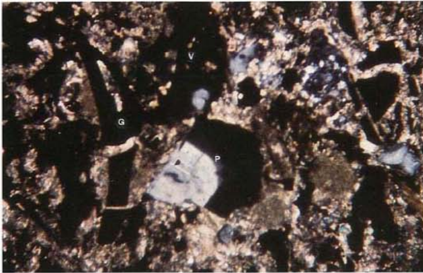
Fig. 7 — Some examples of volcanic glass fragments (G) and zoned plagioclase grain (P) constituting pyroclastic flows of the turbidite sequence of S. Donato Fm. V - volcanicite lithic frg. (0.35 mm long).
