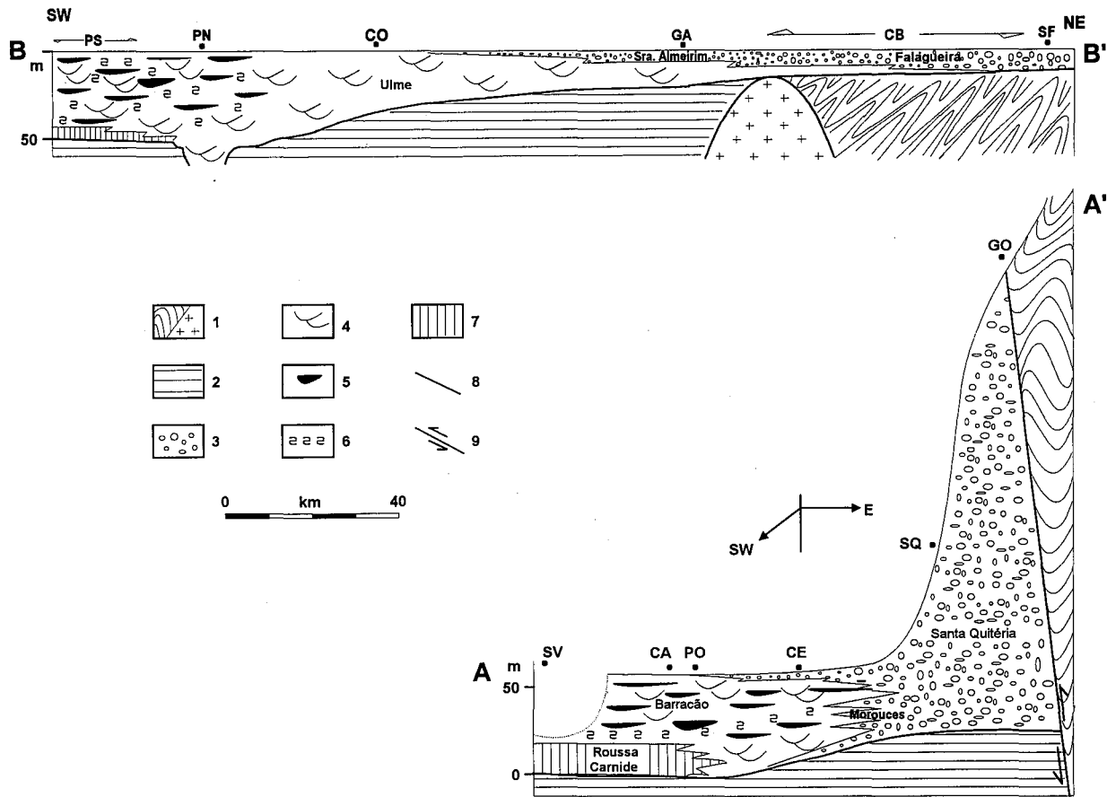
Fig 4 — Schematic geological sections (SW-NE), showing the Upper Pliocene record in the Mondego ( A - A' ) and Lower Tagus ( B - B' ) Tertiary basins. 1 - basement (metamorphosed / granitic); 2 - Mesozoic and Cenozoic substratum; 3 - alluvial conglomerates; 4 - alluvial sandstones; 5 - alluvial mudstones; 6 - marsh and swamp sediments; 7 - marine sandstones; 8 - sedimentary discontinuity; 9 - Lousã fault; SV - Senhora da Vitória beach (S. Pedro de Muel); CA - Carnide; PO - Pombal; CE - Cernache (Coimbra); SQ - Santa Quitéria; GO - Góis (Carvalho and Sacões sections); PS - Setúbal peninsula; PN - Pinhal Novo; CO - Coruche; GA - Gavião; CB - Castelo Branco region; SF - Spanish frontier.
