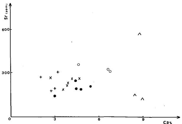
Fig.10 — Diagrama Sr (ppm)-Ca (%).
